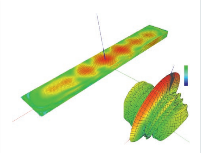
E-field visualization and accurate OTA beam pattern measurement for AAS.
